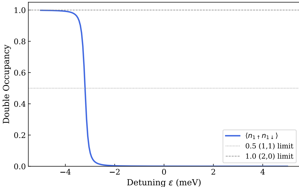
Double Occupancy on Dot 1 vs Detuning
