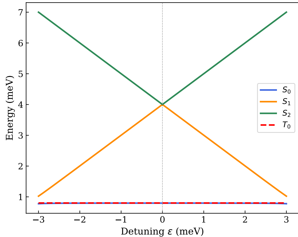
Singlet/Triplet Spectrum vs Detuning
