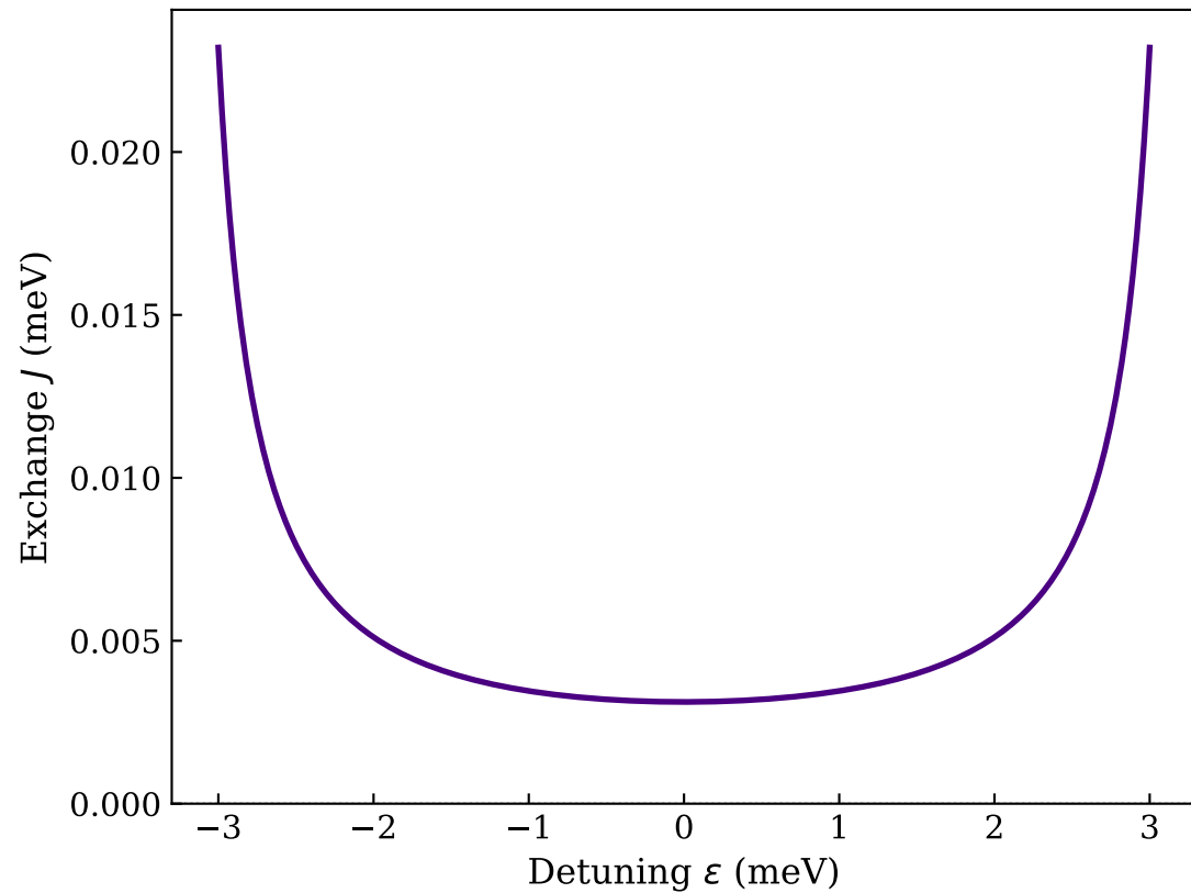
Exchange Splitting J(\varepsilon)
