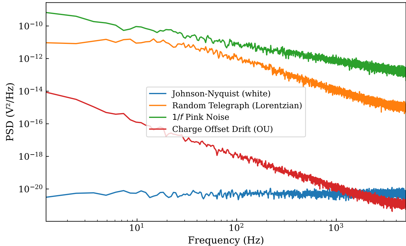
Noise Power Spectral Densities
