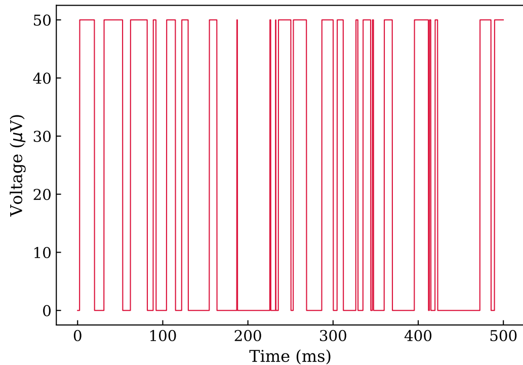
RTN Time Trace
