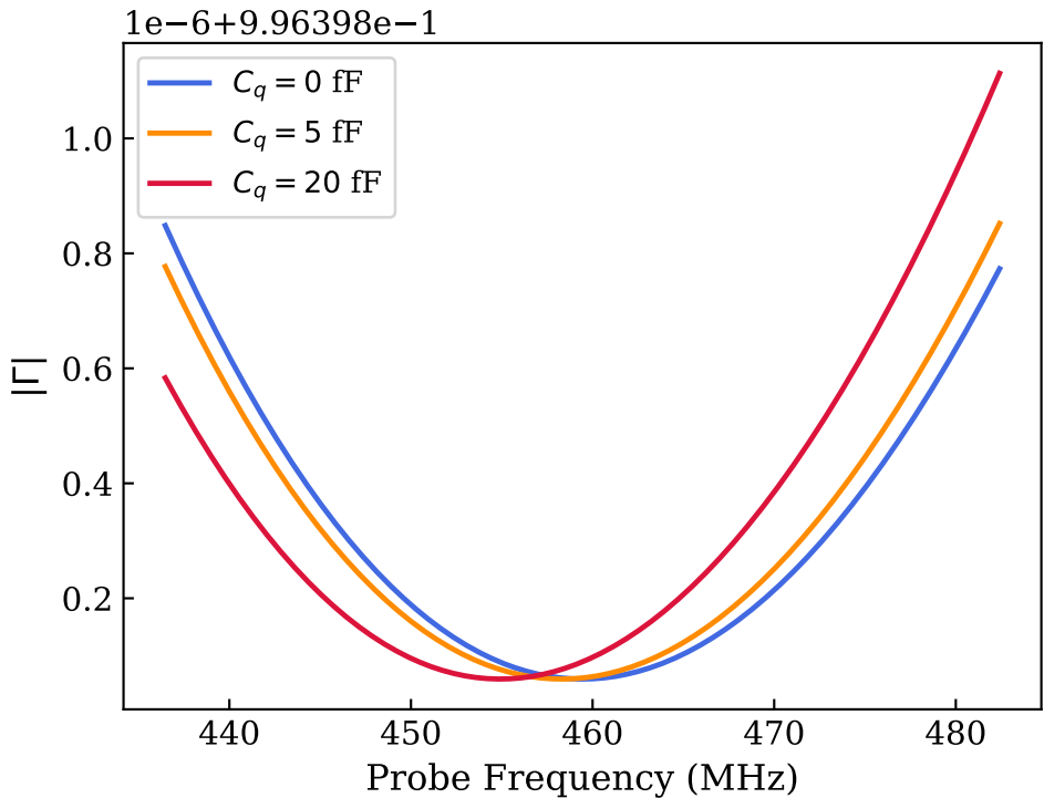
Reflection Amplitude vs Frequency
