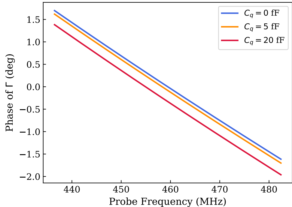
Reflection Phase vs Frequency
