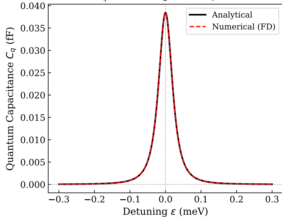
C_q vs Detuning ( t = 15 \mu\text{eV} )
