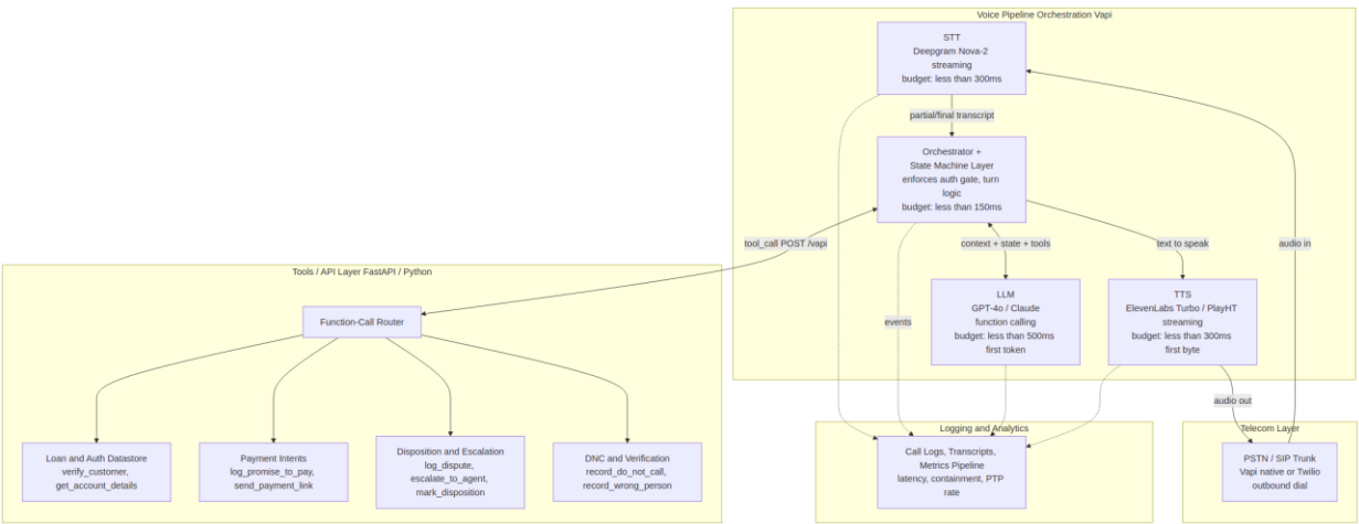
Figure 1. End-to-end pipeline: telephony, voice pipeline, tools/API layer, and observability.
