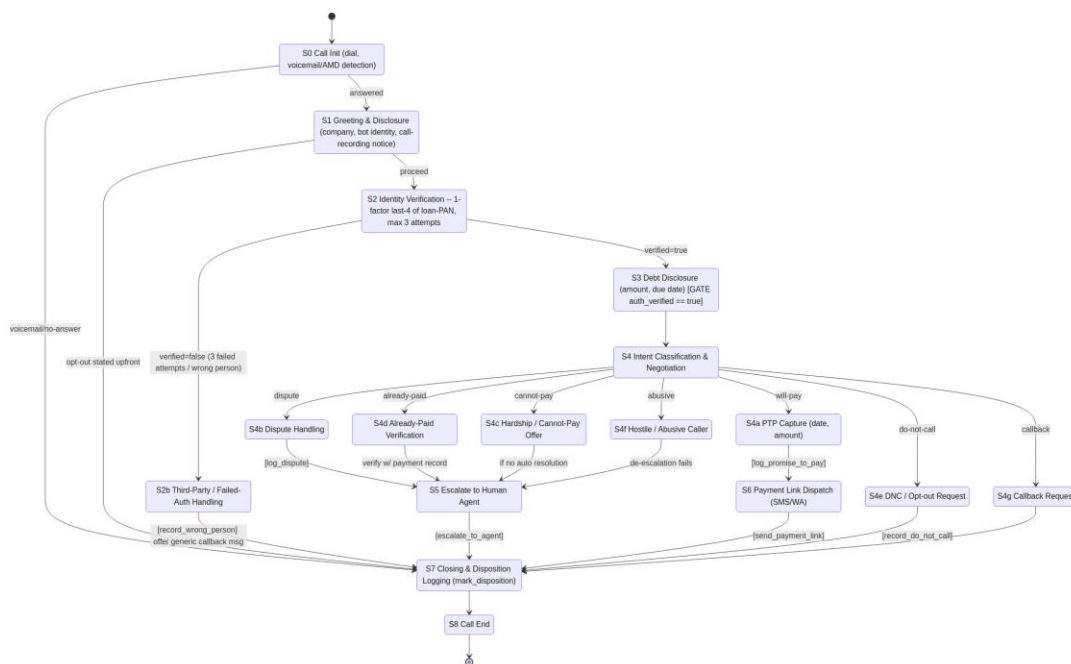
Figure 2. Full state machine. Double-bordered states are code-enforced gates.
