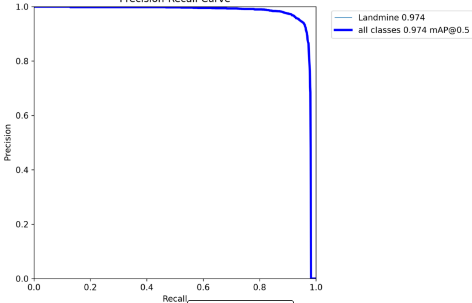
Precision-Recall Curve
