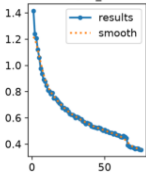
val/cls_loss
