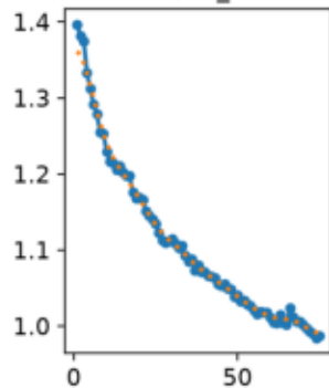
val/df_l_loss
