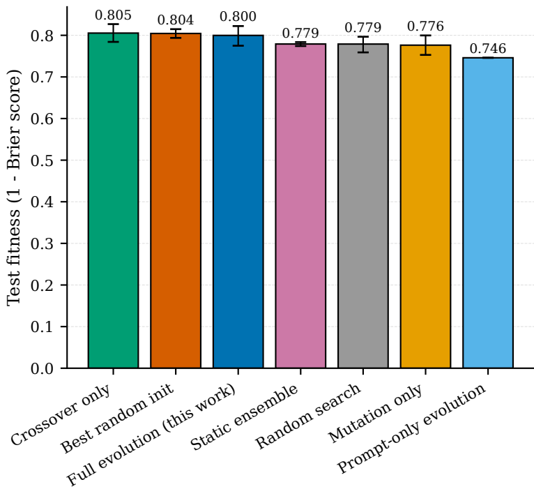
Test fitness by method (mean \pm 95% CI)
