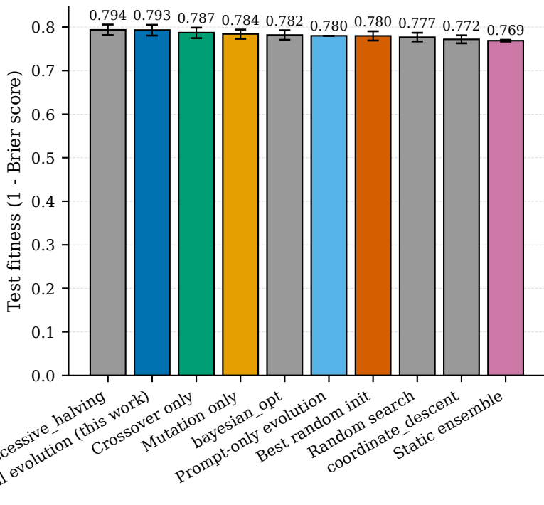
Forecasting test fitness by method
