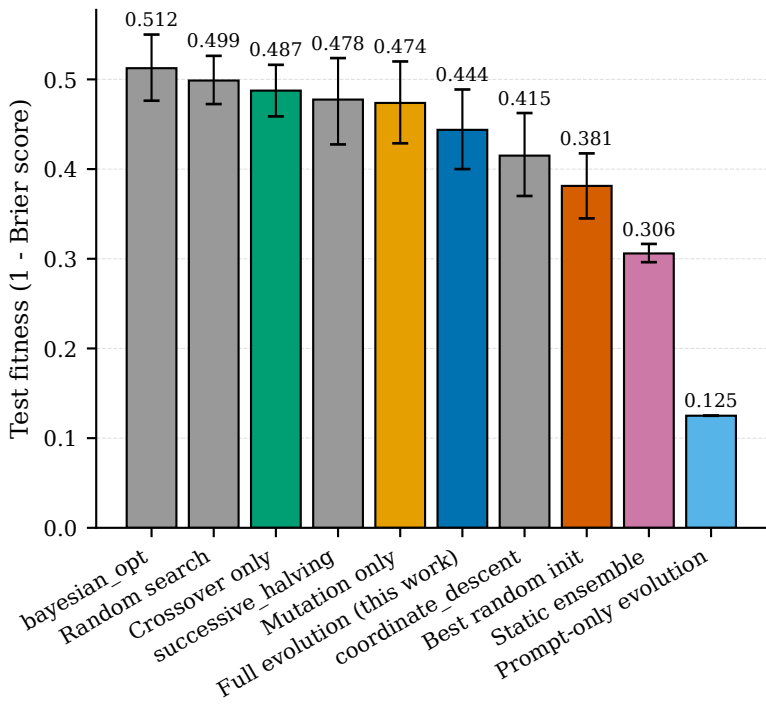
Knowledge test fitness by method
