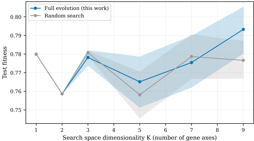
Decisive dimensionality sweep -- forecasting
