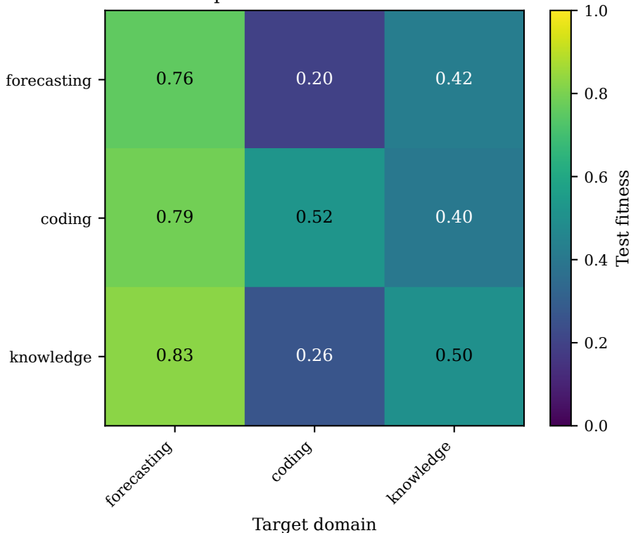
Champion cross-domain transfer
