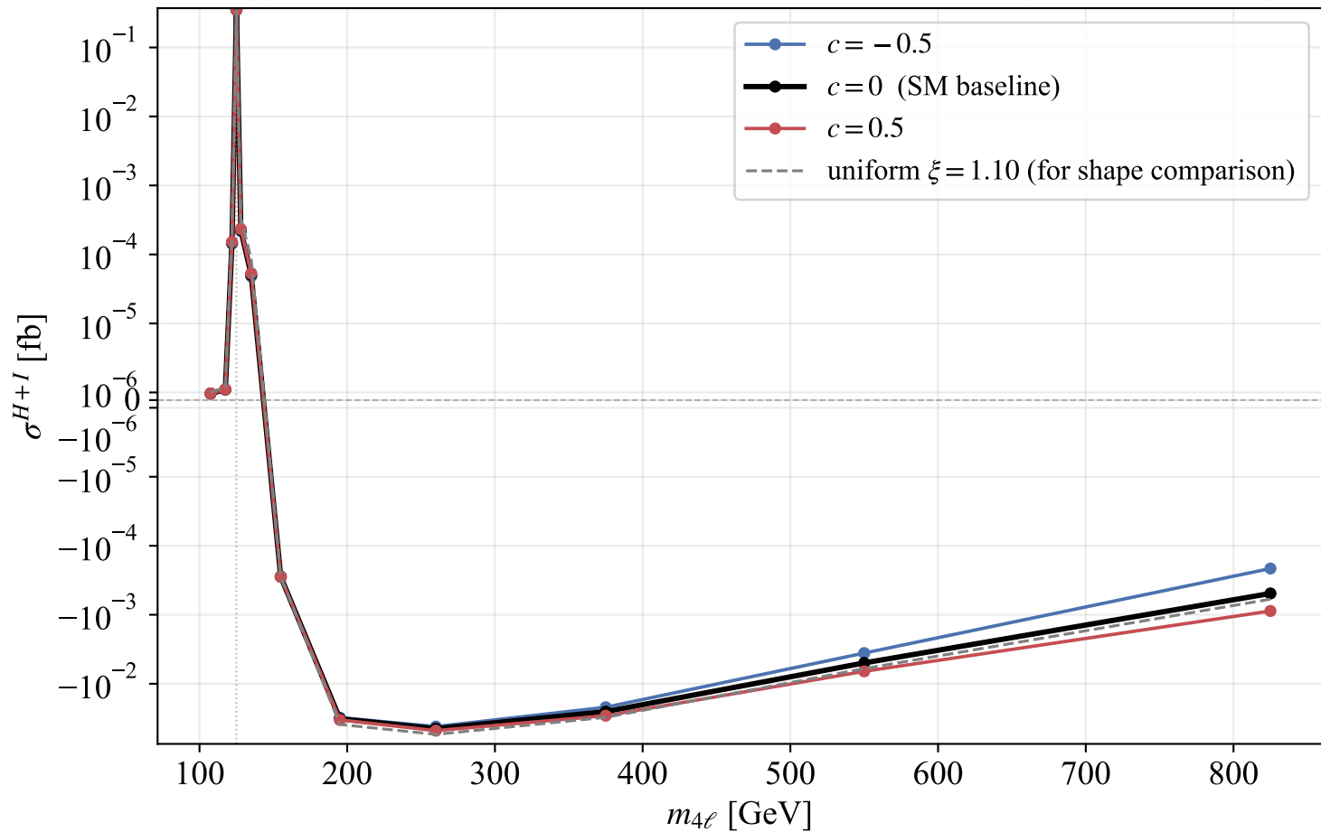
Higgs-related lineshape: \xi(m) = 1 + c(m/1\text{ TeV})^2 toy EFT coupling
