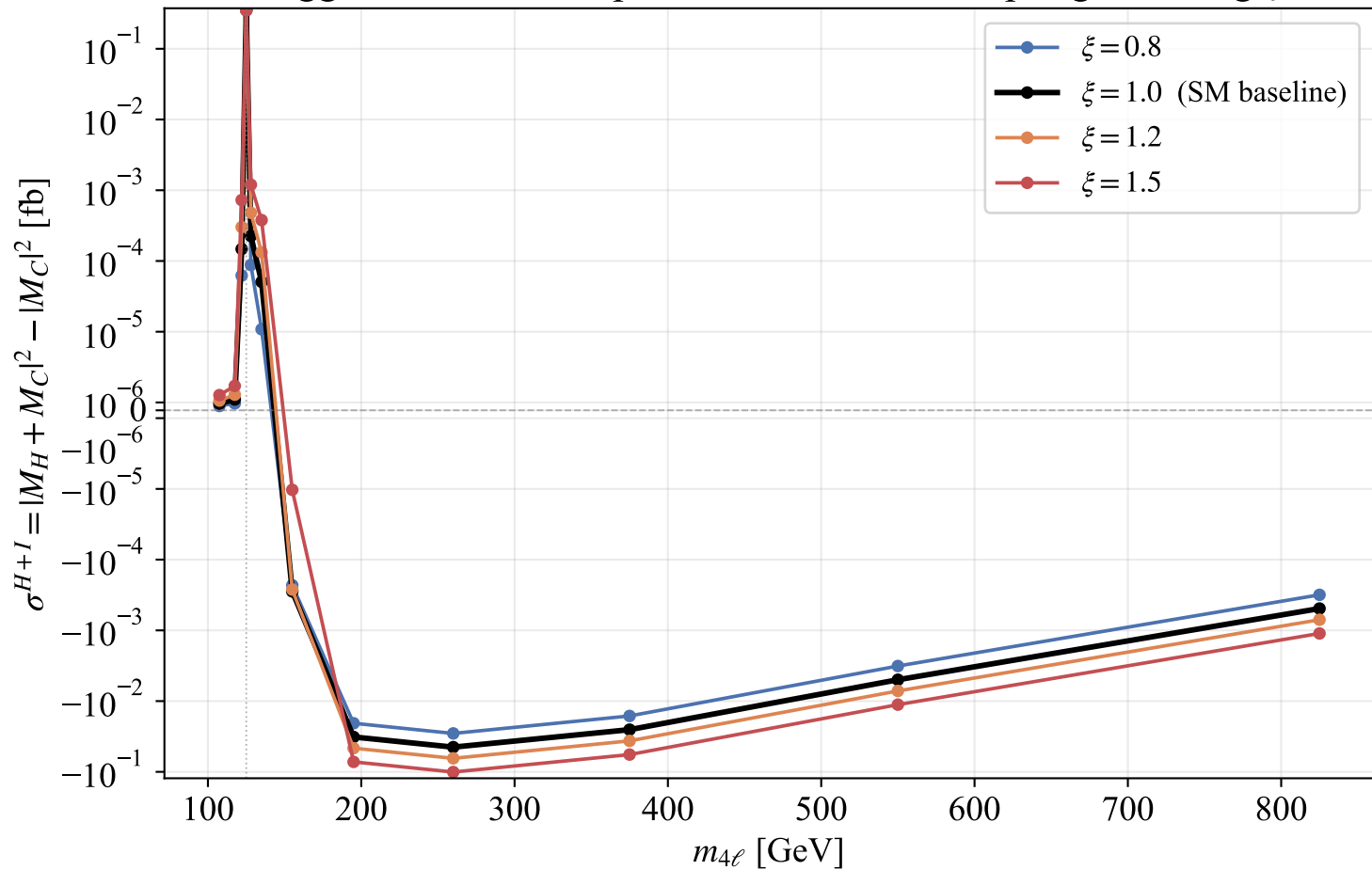
Higgs-related lineshape under a uniform coupling rescaling \xi
