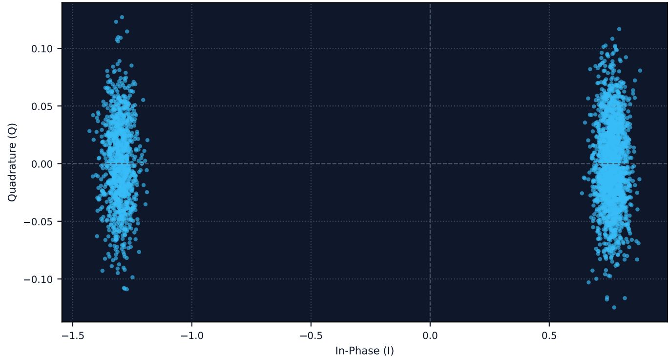
Demodulated Baseband Constellation Diagram — [WBFM]
