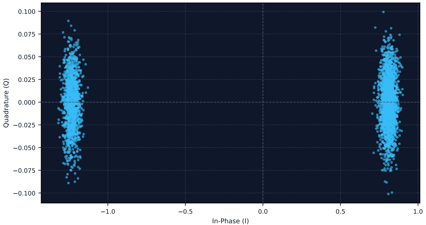
Demodulated Baseband Constellation Diagram — [BPSK]
