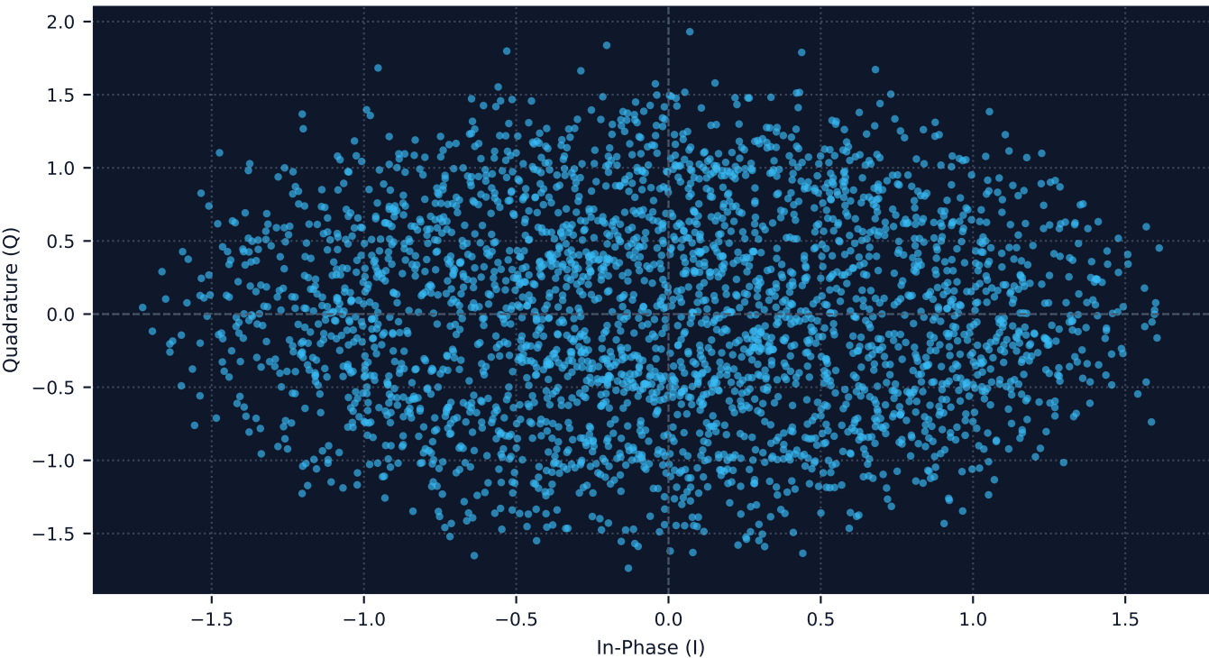
Demodulated Baseband Constellation Diagram — [16-QAM]
