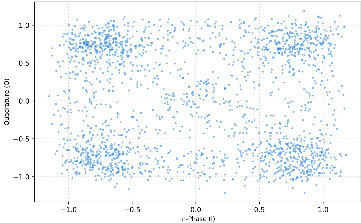
Demodulated Baseband Constellation Diagram (QPSK)
