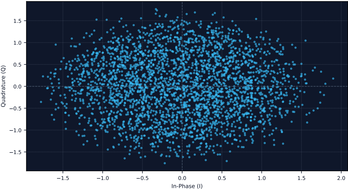
Demodulated Baseband Constellation Diagram — [64-QAM]
