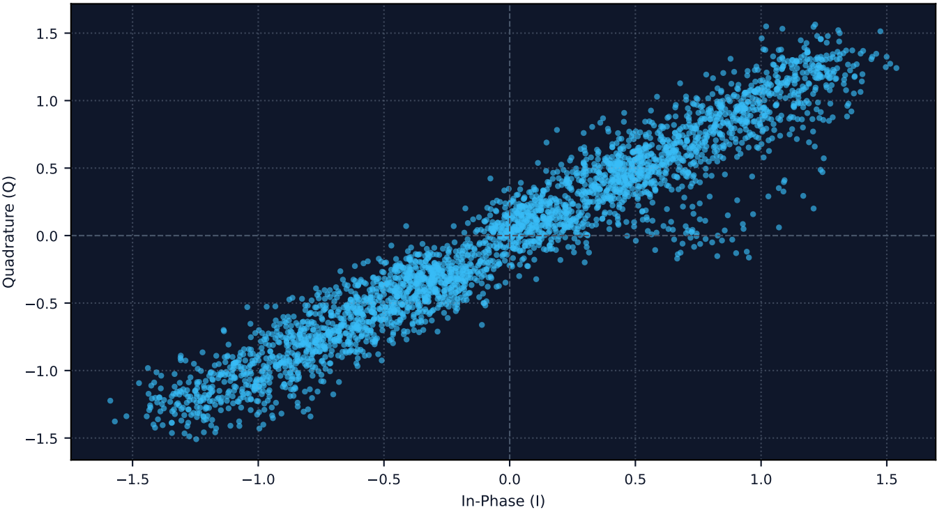
Demodulated Baseband Constellation Diagram — [AM-DSB]
