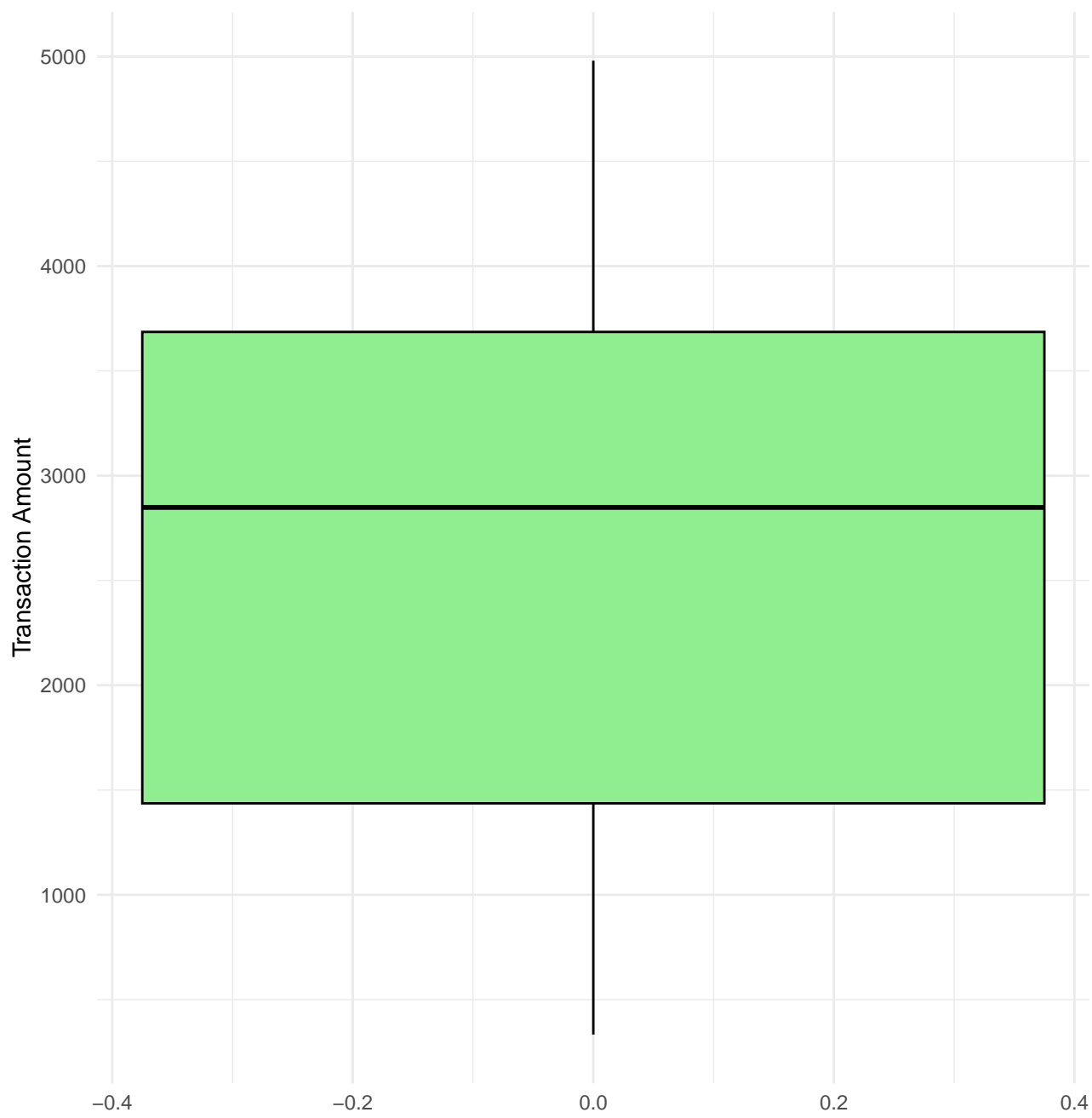
Boxplot of Transaction Amounts
