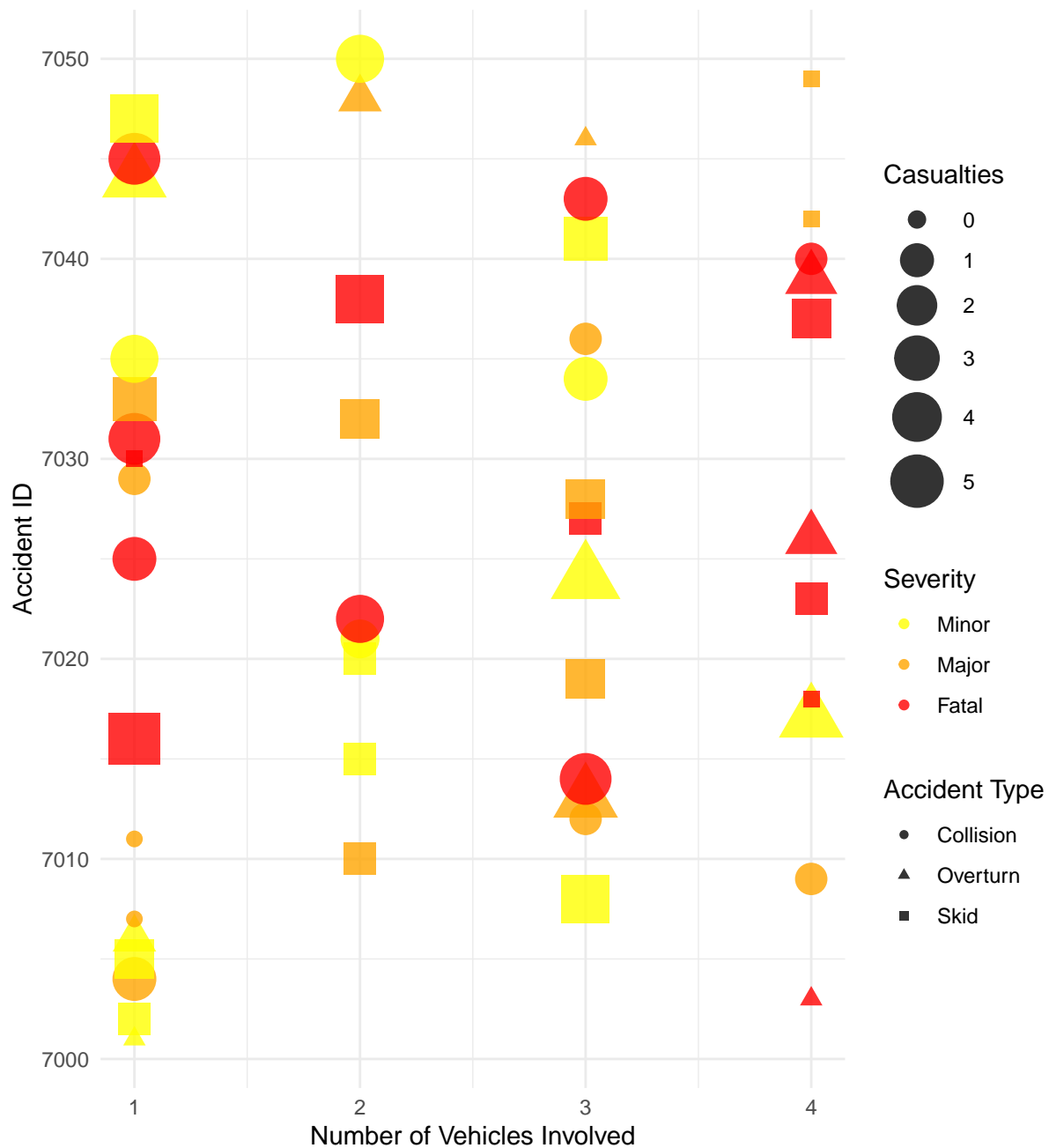
Visual Encoding of Traffic Accident Data
