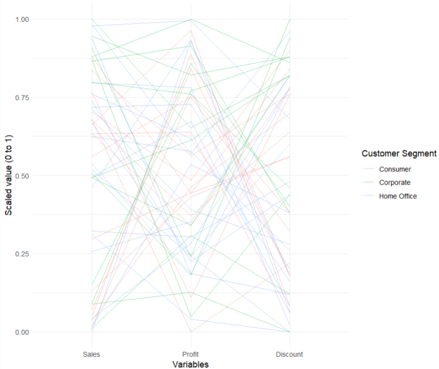
Parallel Coordinate Plot (Sales, Profit, Discount)
