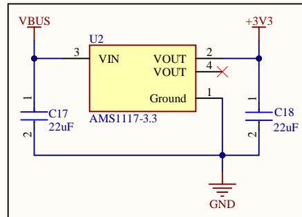
STM32 Microcontroller - Power
