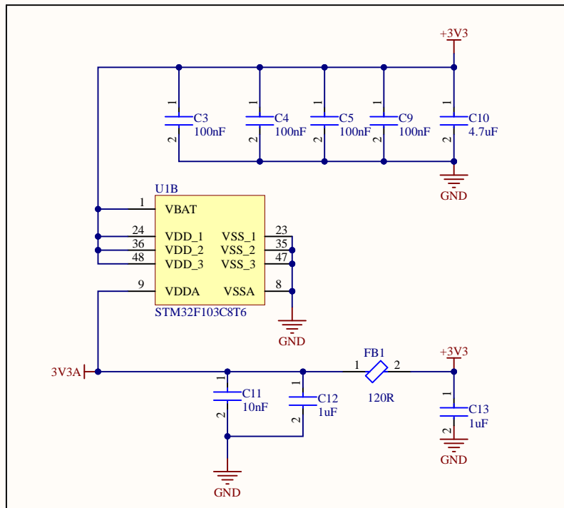
STM32 Microcontroller - Power
