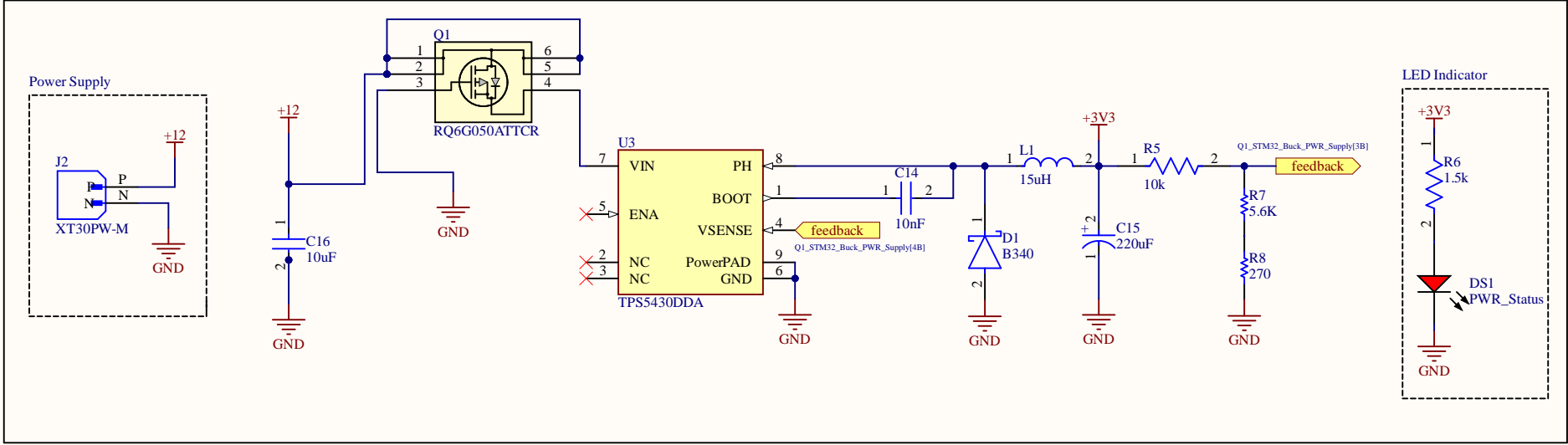
Power Supply and Circuit Protection
