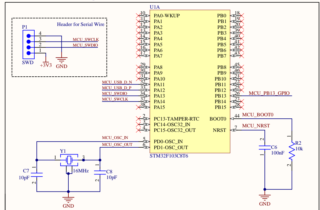
STM32 Microcontroller - Peripherals
