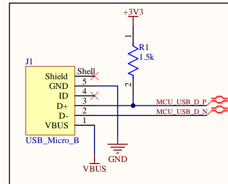
USB Micro B Connector
