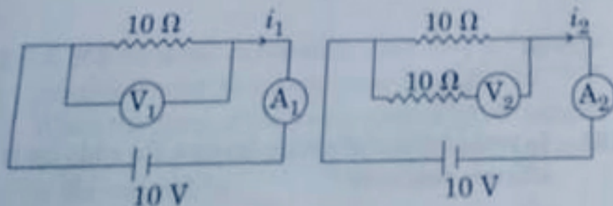
Circuit 2
