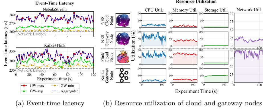
Fig. 3: Latency and resource utilization results of the experiment
