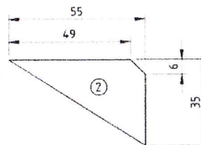
DETAIL BRACKET
