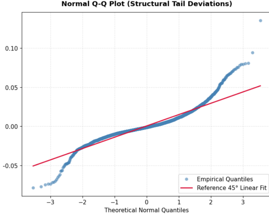
Figure 2.2: Normal Q-Q plot showing tail deviations.
