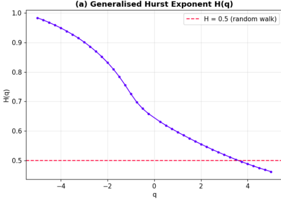
Figure 2.8: Generalised Hurst Exponent H(q) from MF-DFA.
