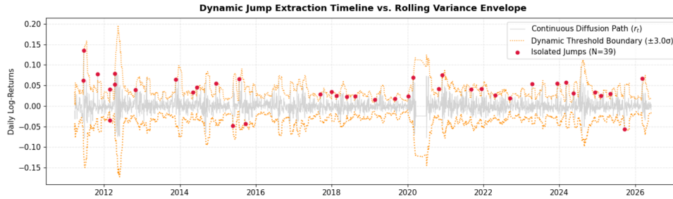
Figure 2.5: Dynamic jump extraction timeline (rolling 3\sigma corridor and detected jumps).
