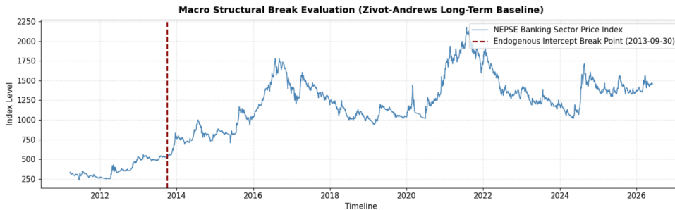
Figure 2.6: Macro Structural Break Evaluation (Zivot-Andrews Long-Term Baseline).
