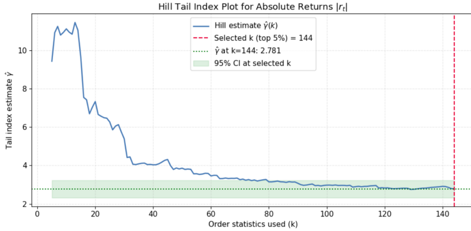
Figure 2.7: Hill tail index plot for absolute returns |r_t| (stability over k ).
