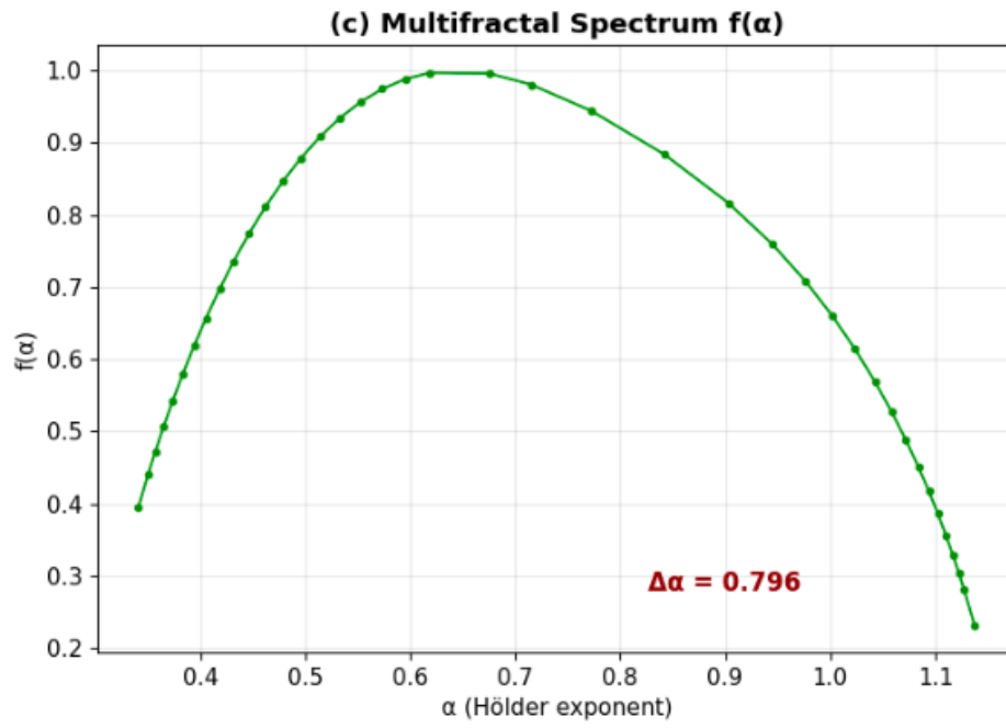
Figure 2.9: Multifractal spectrum \alpha vs. f(\alpha) from MF-DFA.
