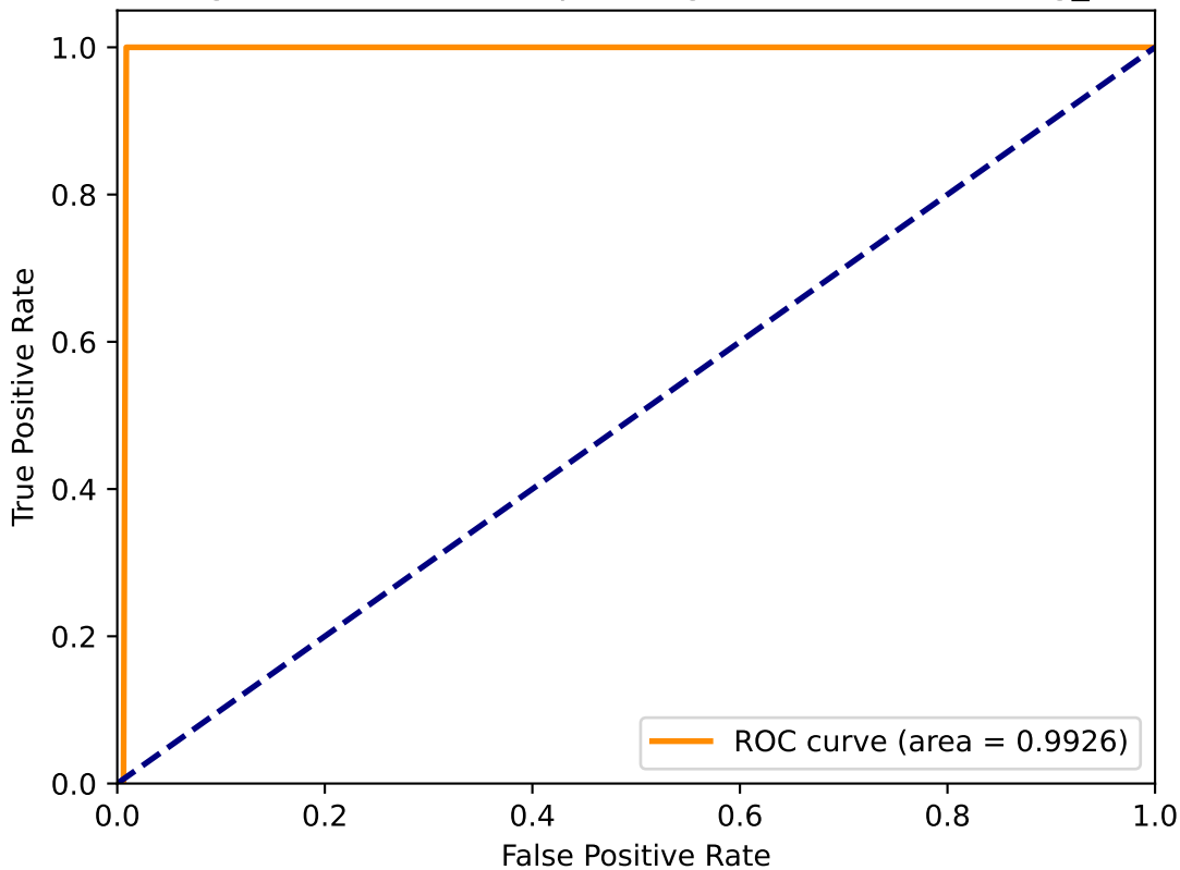
Augmented Receiver operating characteristic of ecg_7
