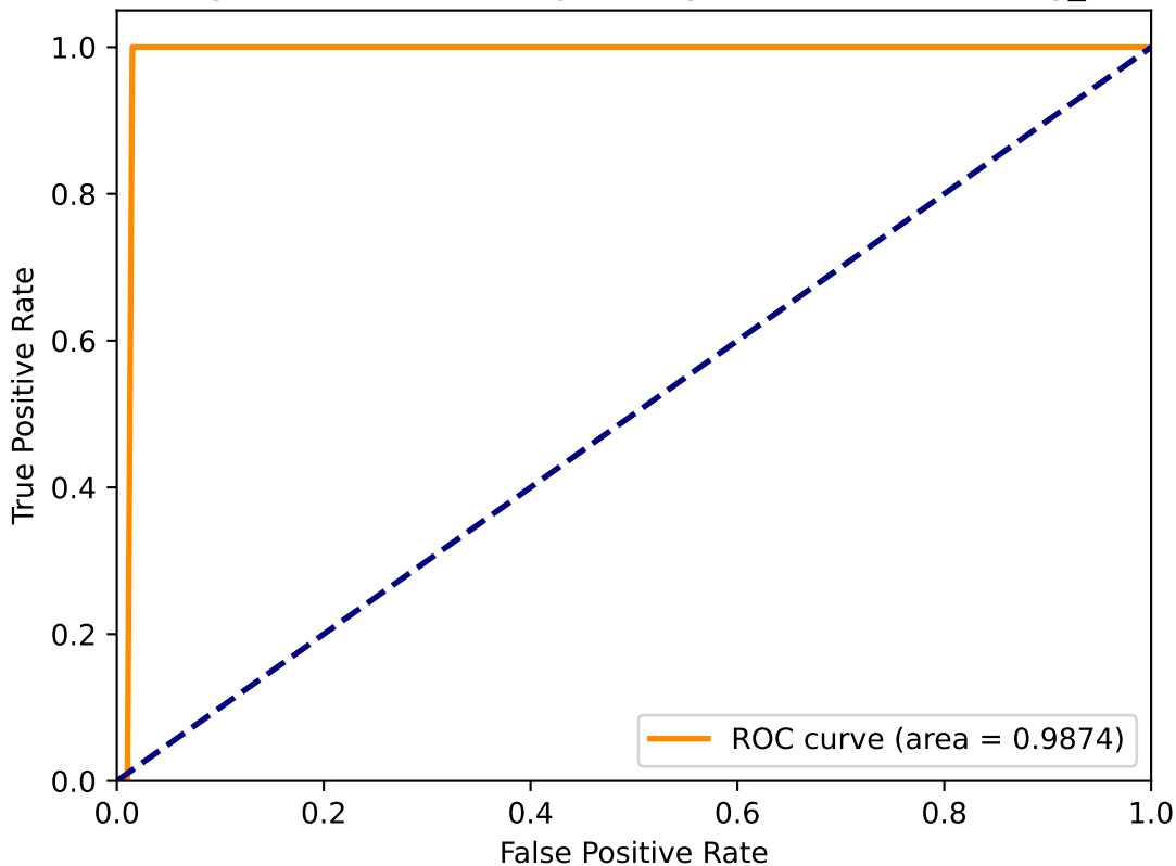
Augmented Receiver operating characteristic of ecg_6
