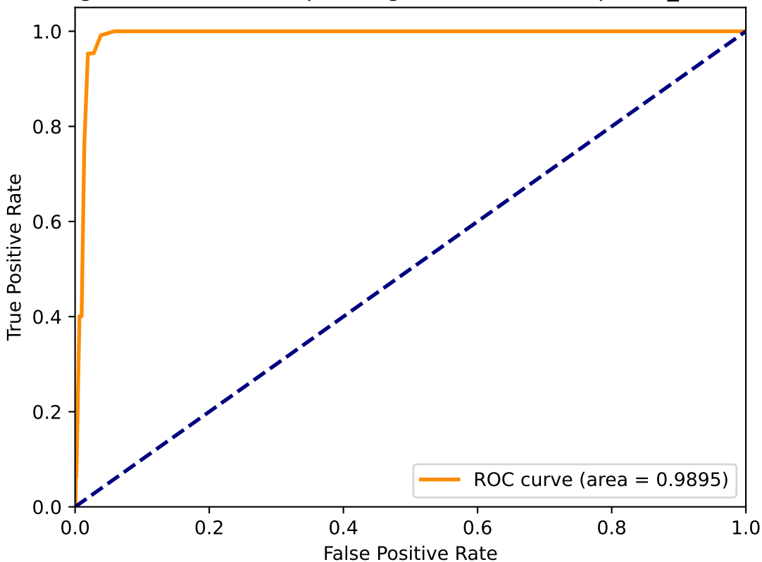
Augmented Receiver operating characteristic of power_demand
