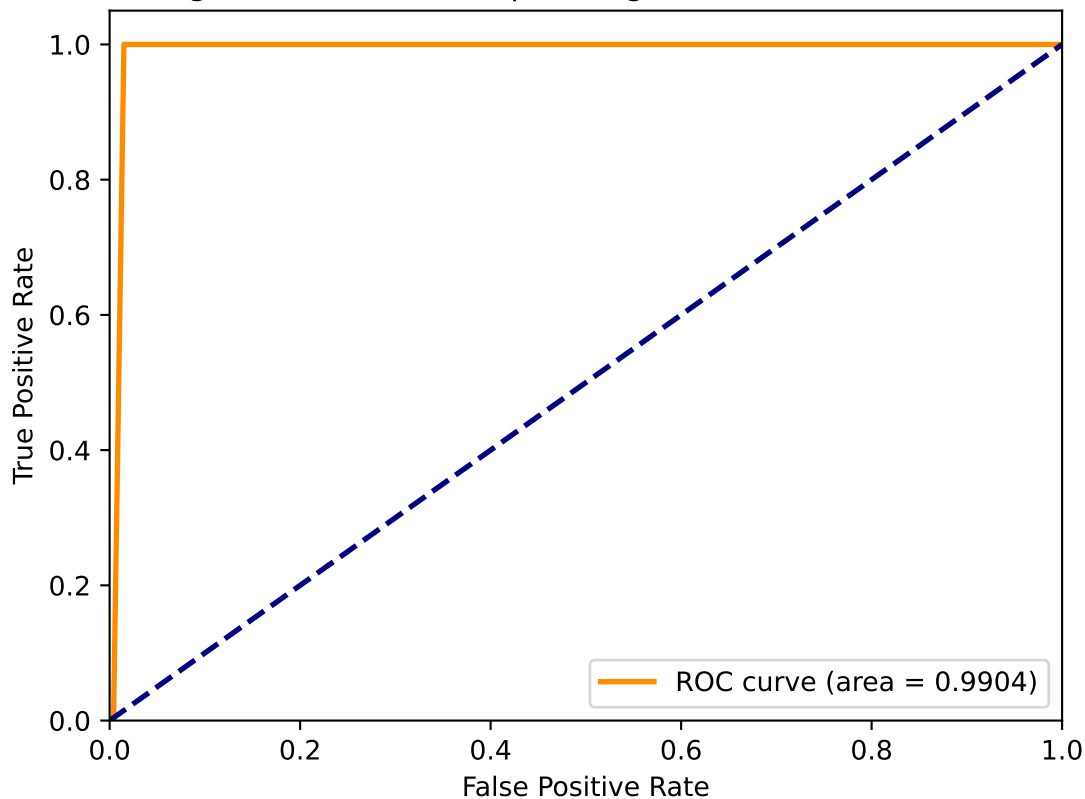
Augmented Receiver operating characteristic of TEK17
