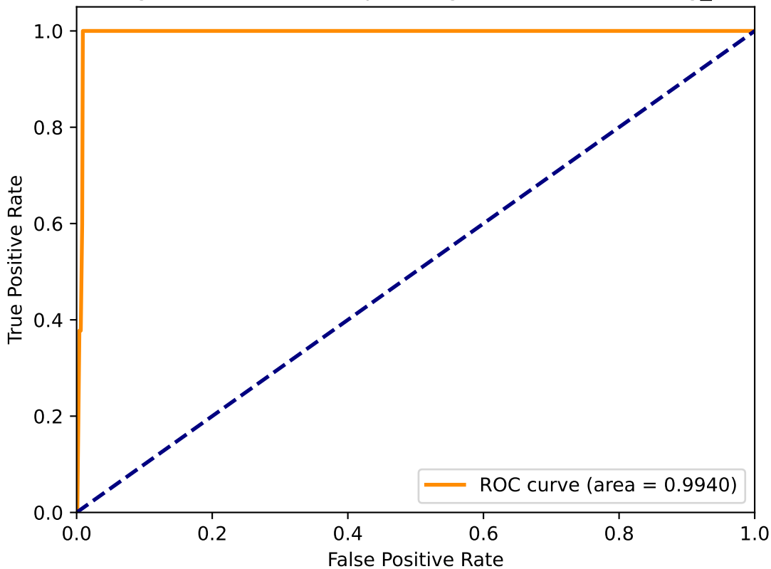
Augmented Receiver operating characteristic of ecg_9
