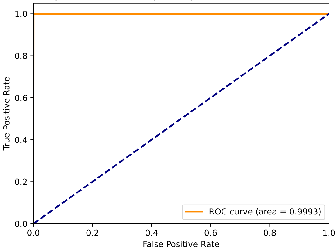
Augmented Receiver operating characteristic of SWAT16
