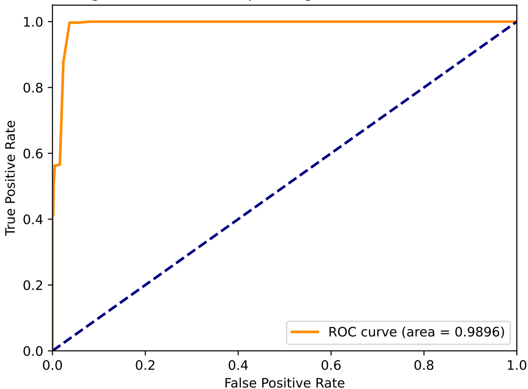
Augmented Receiver operating characteristic of TEK14
