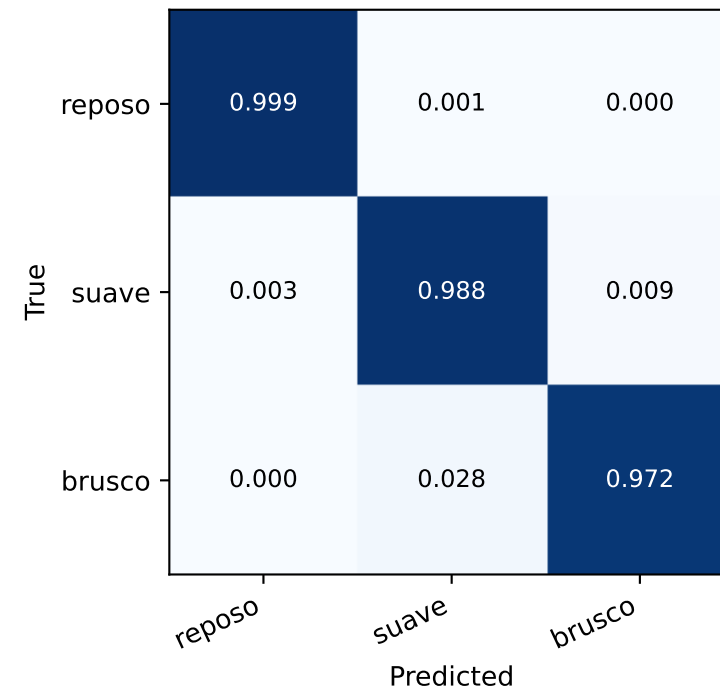
Random Forest compact
