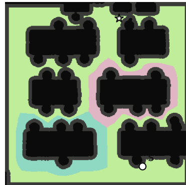
(f) arc-smoothed path, R \geq 0.8 m
