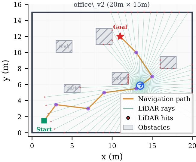
Fig. 3. Mock backend visualization: autonomous navigation in the office_v2 scene. The robot (blue) follows a planned path (orange) while 360° LiDAR rays (green) detect obstacles. This zero-dependency simulation runs on any machine without GPU or ROS2.
