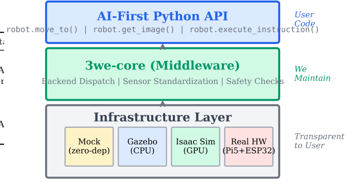
Fig. 2. Three-layer architecture. Users write Python against the AI-First API (top). The middleware dispatches to one of four backends (bottom) with identical semantics. ROS2 infrastructure is fully transparent.
