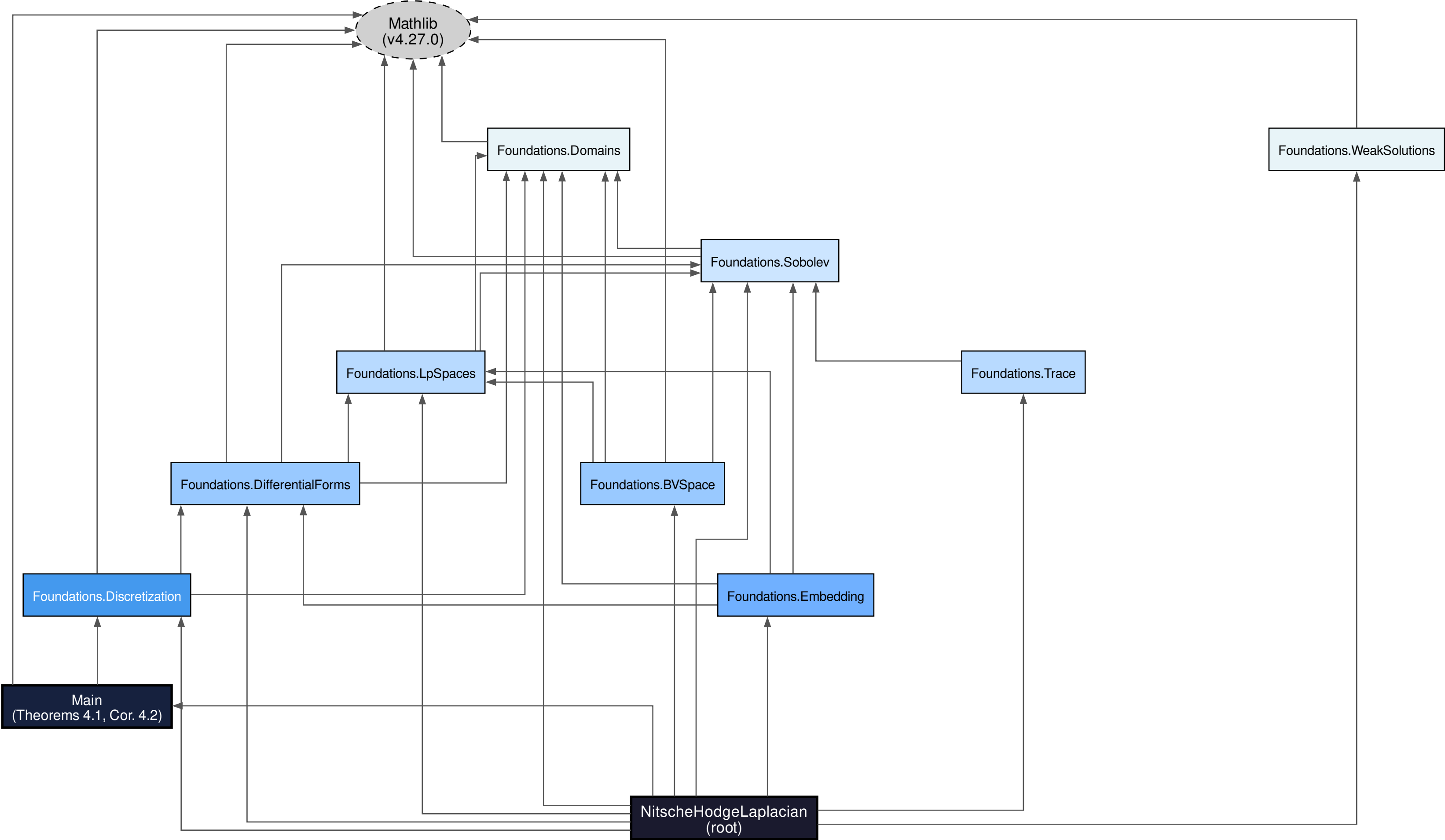
NitscheHodgeLaplacian — Module Import Graph (Lean 4 / Mathlib v4.27.0)
