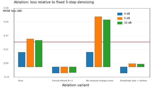
Fig. 3. Ablation on residual-change score and forced refresh.
