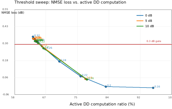
Fig. 1. Preliminary threshold sweep from the surrogate sparse-DD harness.
