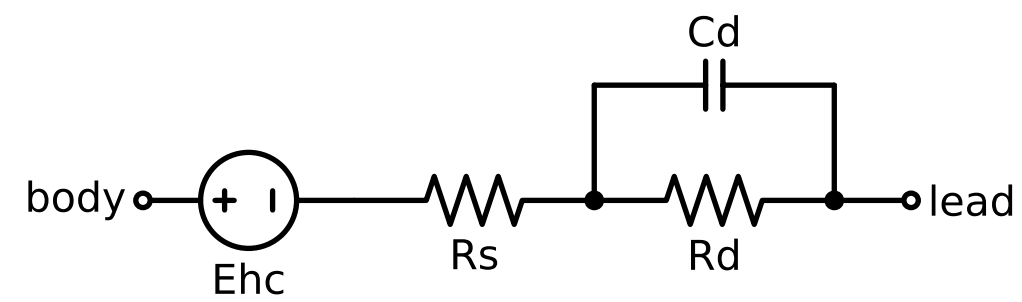
Skin-electrode model (LA, RA and RL)
