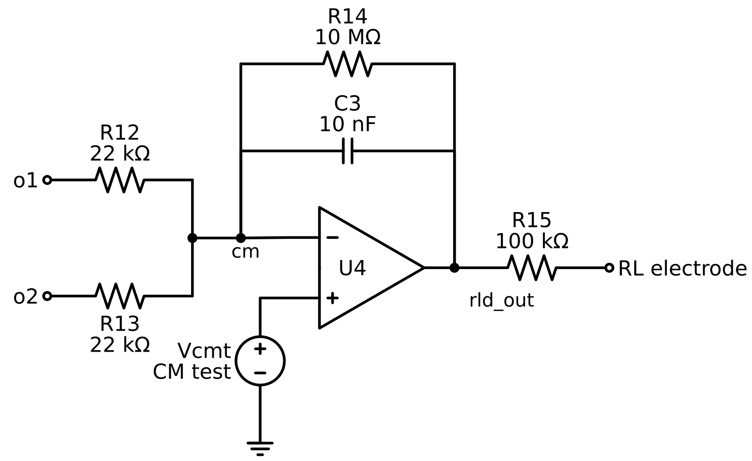
Driven right leg
