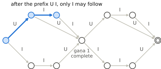
(b) Minimal DAWG, same lines: 11 states, 14 edges
