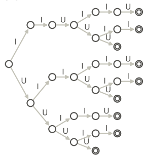
(a) Trie of the 9 lines: 29 states
