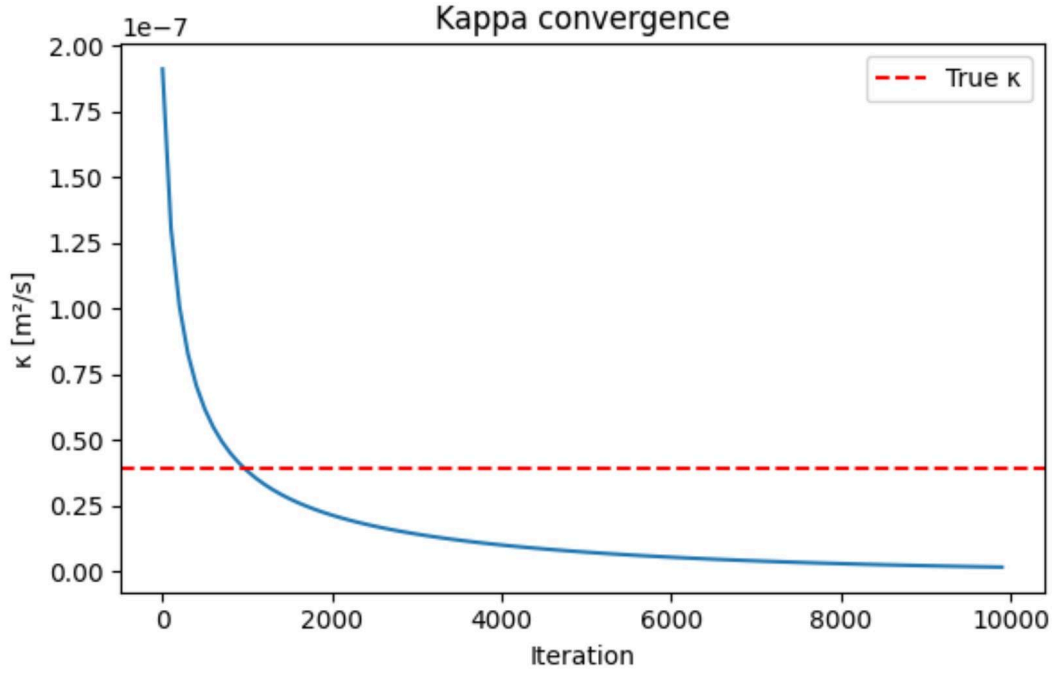
Fig. 12. Representative \kappa trajectory for the 2D axisymmetric inverse PINN . The recovered diffusivity decays monotonically past the Spohn et al. reference (dashed line) toward zero, indicating failure to converge. The dashed red line marks Spohn's \kappa = 3.93 \times 10^{-8} .
