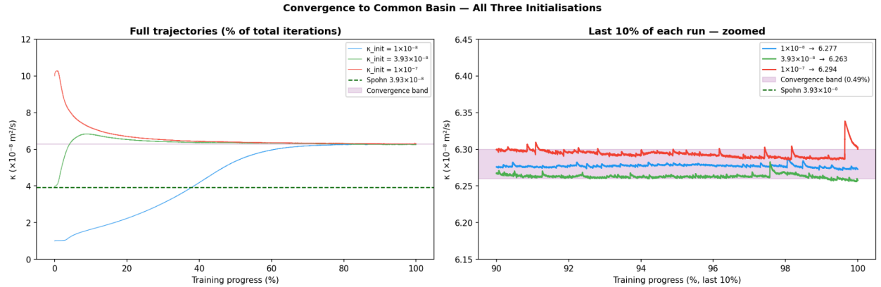
Fig. 7. Left: all three trajectories normalised to training progress (%). Right: final 10% of each run zoomed to show convergence. Purple band marks the convergence region ( 6.26 - 6.30 \times 10^{-8} \text{ m}^2/\text{s} , width 0.49%)
