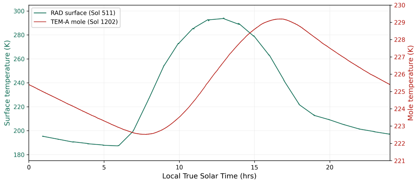
Fig. 2. Diurnal temperature records used as PINN inputs: RAD surface temperature (Sol 511, left axis) and TEM-A mole temperature (Sol 1202, right axis). The amplitude attenuation from \sim 107 K at the surface to \sim 6.7 K at mole depth, and the phase lag between the two signals, are the observational signatures from which \kappa is recovered.
