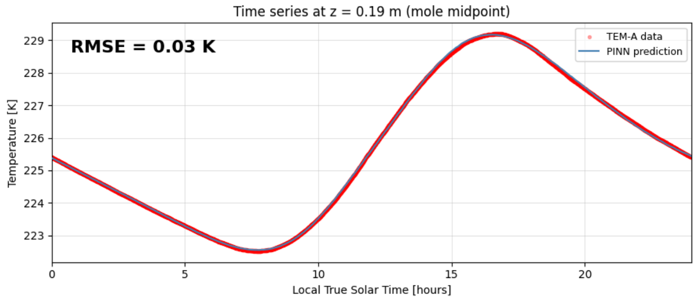
Fig. 11. 2D axisymmetric forward PINN prediction at the mole midpoint ( z = 0.19 m) compared with TEM-A data. RMSE = 0.03 K.
