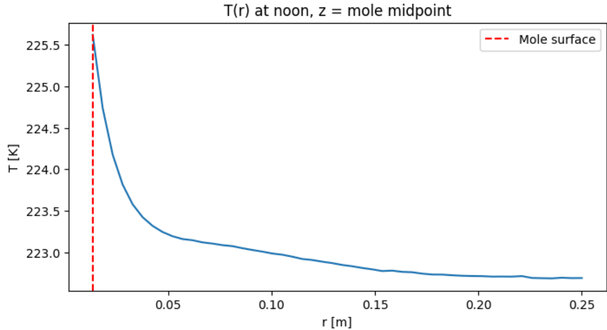
Fig. 10. Radial temperature profile T(r) at the mole midpoint depth at noon (LTST = 12:00), predicted by the 2D axisymmetric forward PINN. The dashed red line marks the mole surface ( R_{\text{mole}} = 1.35 cm). Temperature decays sharply within the first \sim 5 cm from the hull and approaches the undisturbed far-field value by r \approx 15 cm, confirming that the mole's thermal perturbation is localised.
