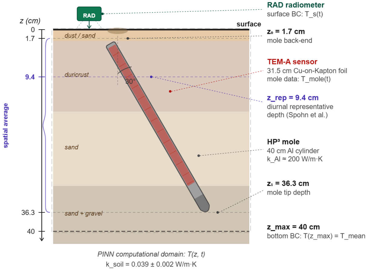
Fig. 1. Cross-section of the HP³ mole in the Martian regolith, showing the PINN computational domain, sensor positions, and the spatial averaging range from z_0 to z_1 . Soil stratigraphy follows Spohn et al. (2024).
