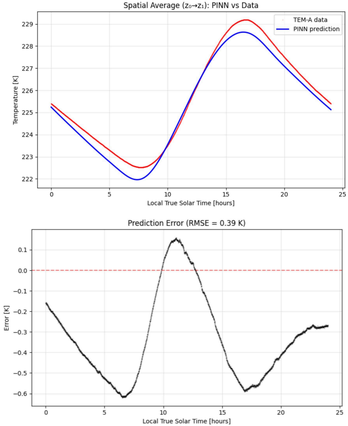
Fig. 6. Spatial average forward PINN results. Top: predicted spatially averaged temperature over [z_0, z_1] compared with TEM-A data, showing the elimination of the phase lag observed in the point-sensor model (cf. Fig. 5.). Bottom: prediction error over one sol, with RMSE = 0.39 K. The residual structure suggests a small remaining model–data mismatch rather than random noise.
