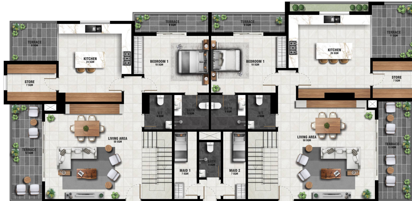
Duplex 2 4 Bedroom 179 sqm
