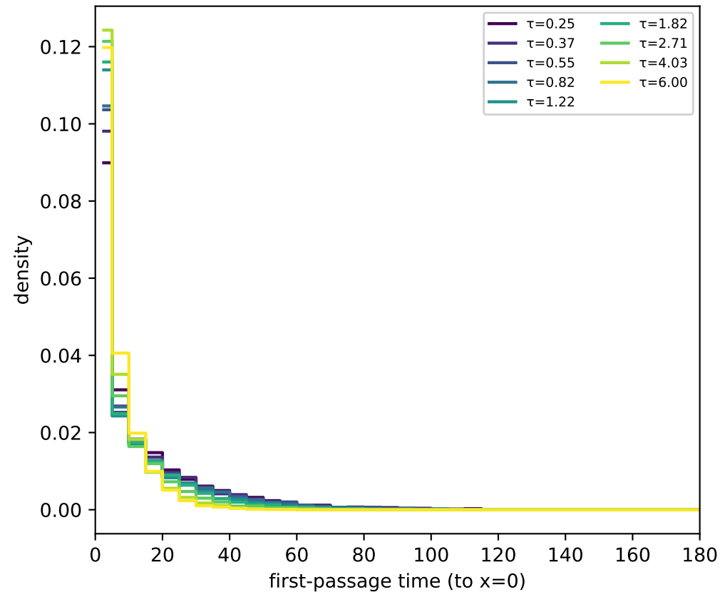
Fig 1 — Engine FPT distributions sharpen & shift left as \tau grows (Corridor1D, fixed sep=6, causal force only)
