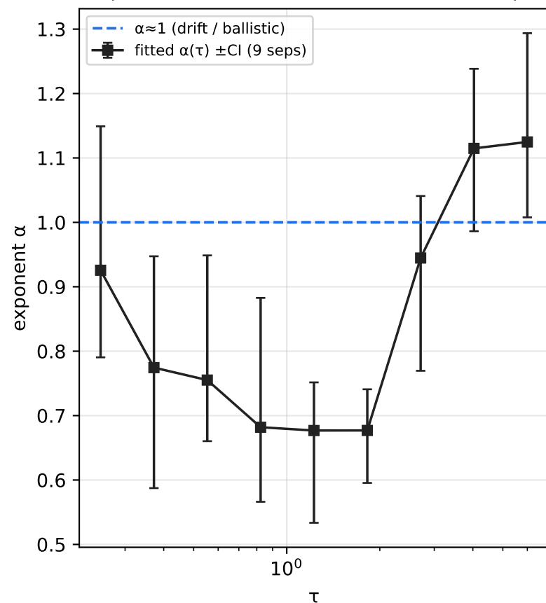
\alpha(\tau) — drift-dominated ( \alpha \approx 1 ) (not the diffusive \alpha=2 of thermal v2)
