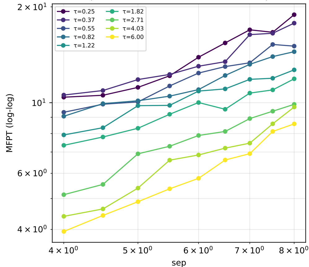
Fig 4 — MFPT(sep) at fixed \tau (log-log) (drift-dominated under causal force)
