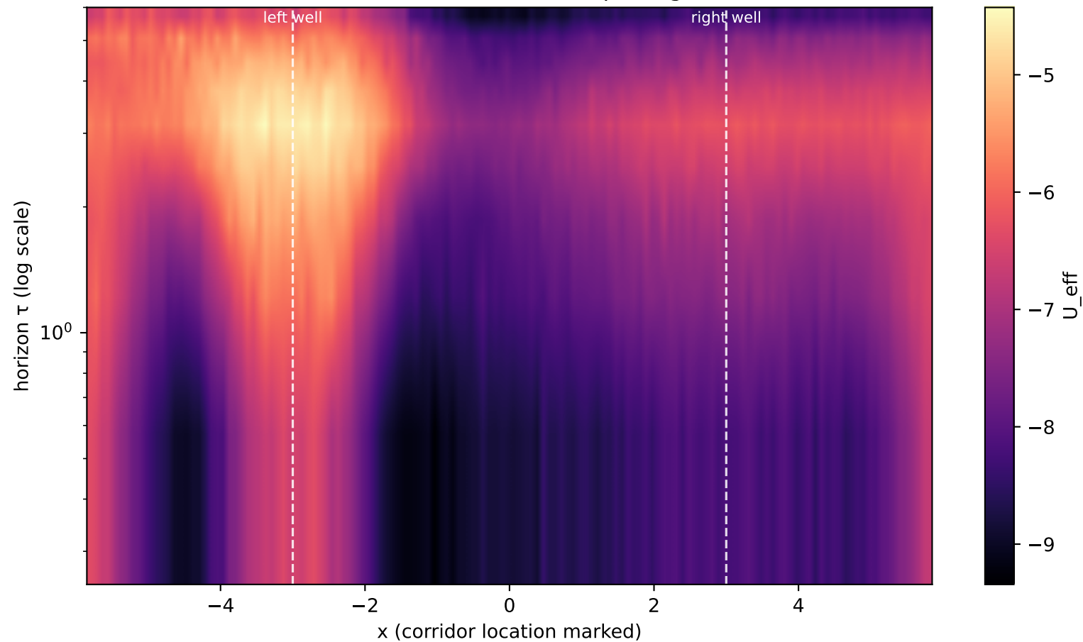
Fig 6 — Effective landscape U_{\text{eff}}(x, \tau) = -\beta T_c S_c(x, \tau) (the dial that moves first-passage)
