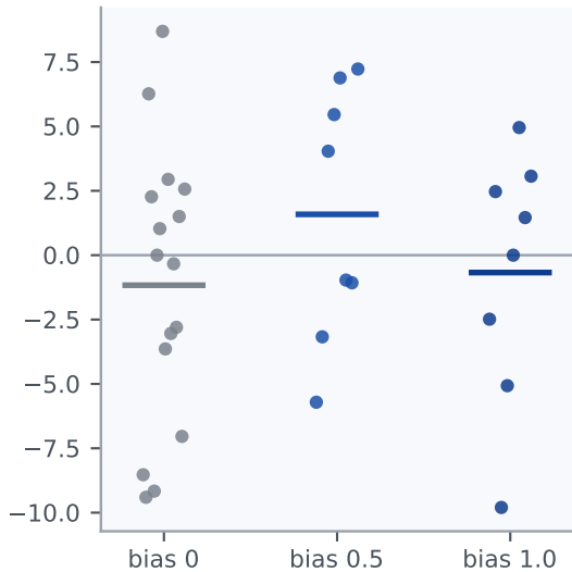
A rotating sampling bias: no circulation
