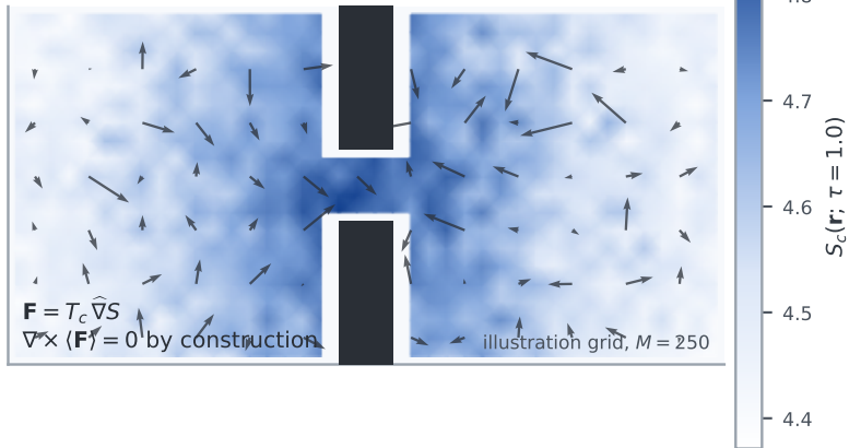
B scalar field, gradient force
