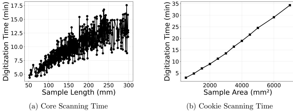
Figure 6: Time to digitize a sample varies by sample type and scanning parameters such as percentage image overlap. Cores scan significantly faster than cookies as they do not need to take images beyond the samples edge. The range of samples included span from a 3 mm x 220 mm core to a 75 mm x 56 mm cookie. The theoretical maximum sample dimensions are limited by the working plane of the machine, approximately 500 mm x 500 mm in our configuration. True sampling times are drastically influenced by configurable machine parameters such as percentage image overlap.
