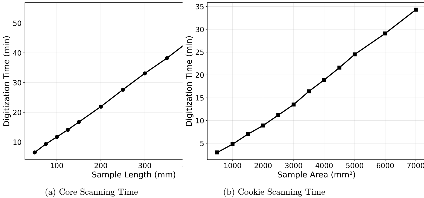
Figure 6: Time to digitize a sample is dependent on the sample’s surface area and the desired final resolution. Cores benefit from linear surface area to sample length. The range of samples included span from a 3 mm x 220 mm core to a 75 mm x 56 mm cookie. The theoretical maximum sample dimensions are limited by the working plane of the machine, approximately 500 mm x 500 mm in our configuration. True sampling times are drastically influenced by configurable machine parameters such as percentage image overlap.
