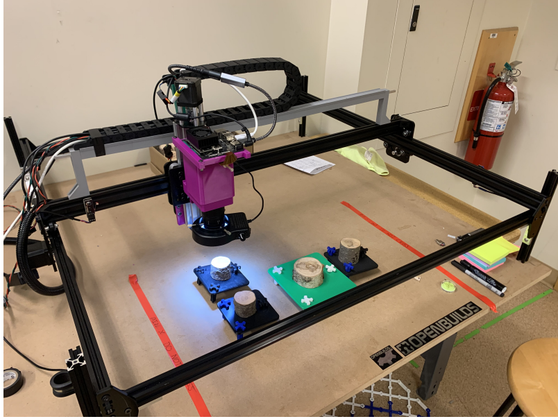
Figure 1: Complete assembly of TIM, shown with a few smaller cookies ready to be scanned. All of the 3D printed parts are available for download on the NIH 3D printing repository (HYPERLINK REMOVED) and the software is open source, with instructions to recreate this tool available on GitHub (HYPERLINK REMOVED). Links to images produced by TIM are provided in Table S3.
