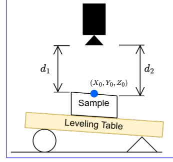
(b) Realistic sample leveling
