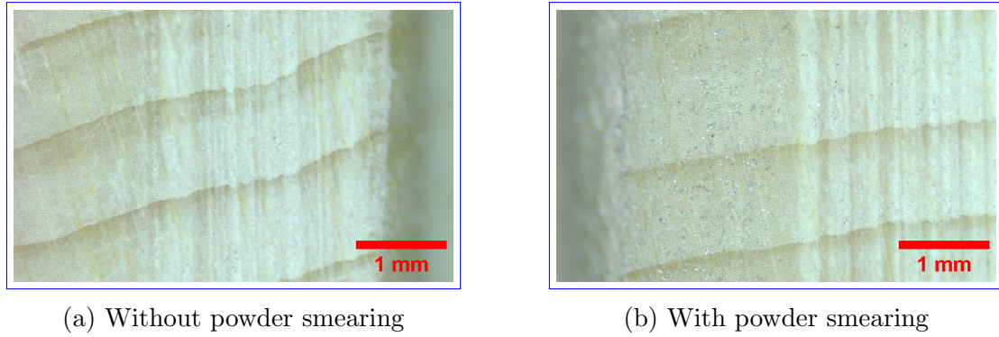
Figure 5: A hard-to-scan sample due significant scratches , with and without silicon carbide smeared on the surface of the core.
