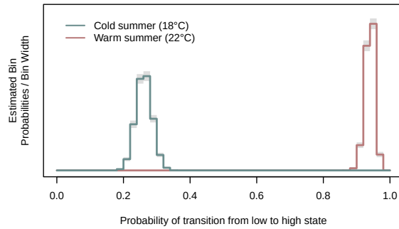
Figure 4: Posterior distributions of transition probability from low to high reproductive states in a cold vs. a warm summer.
