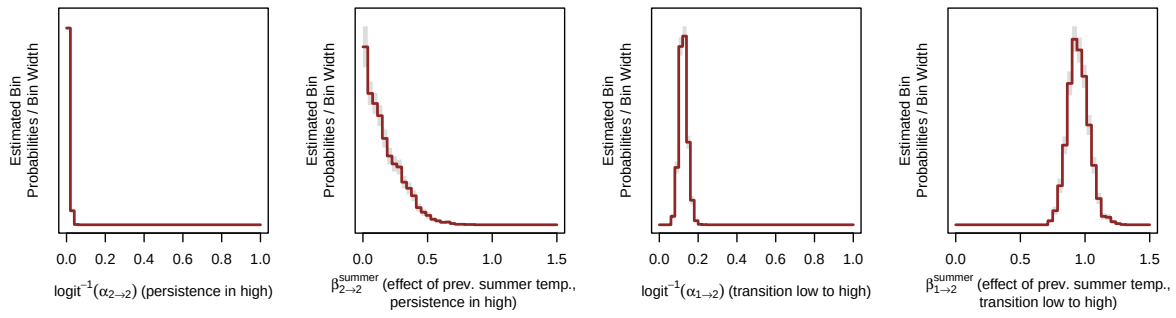
Figure 3: Posterior distributions of the parameters related to state transitions (model with summer temp. on both transitions).
