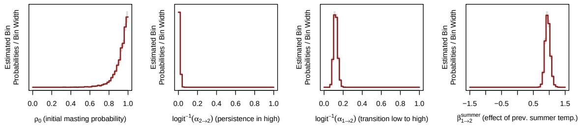
Figure 2: Posterior distributions of the parameters related to state transitions (main text model).
