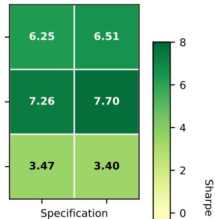
Late fusion
