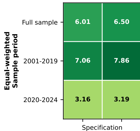
Feature concat
