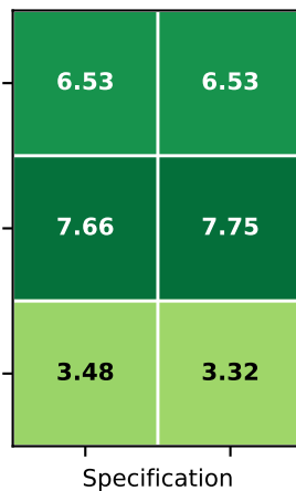
MLP head
