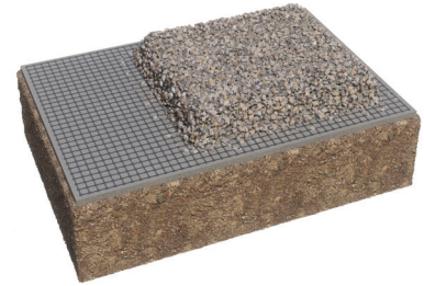
BallastGuard™ with Bedding Material
