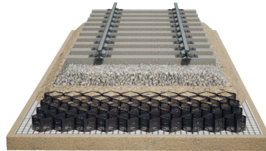
BallastGuard™ with GeoCell
