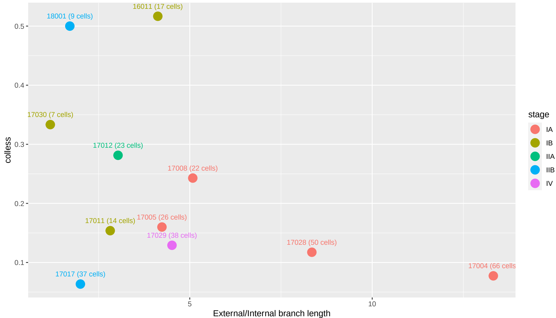
Tree statistics
